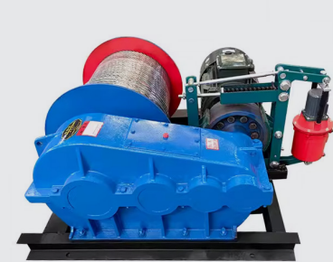
Electric Winch
